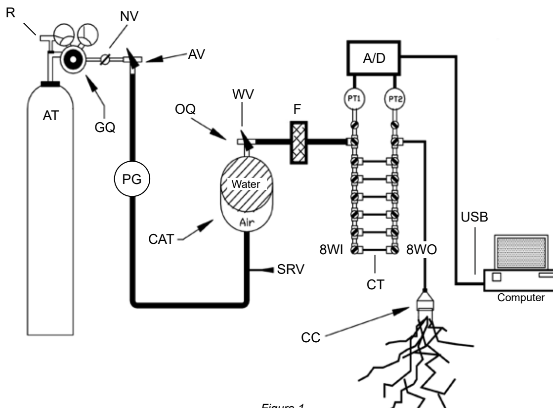
Figure 1 Schematic of High Pressure Flow Meter (HPFM)
